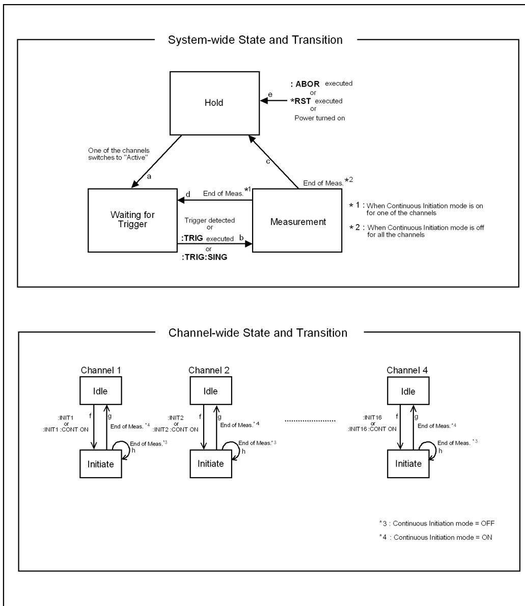
Trigger system
