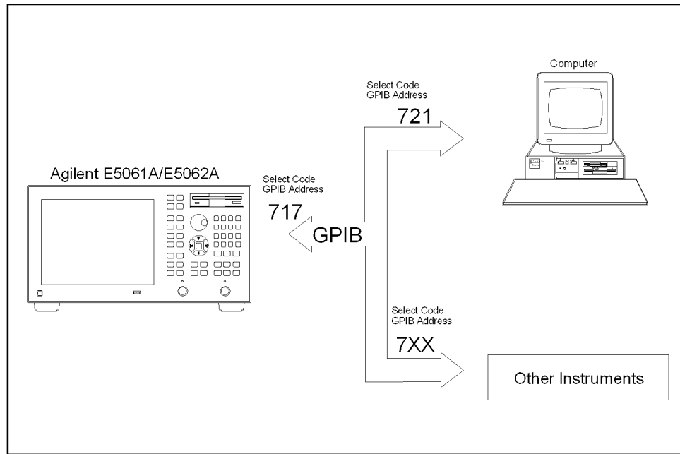
Configuration of the GPIB remote control system
